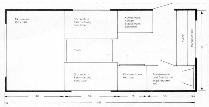
Grundriss Hilton
